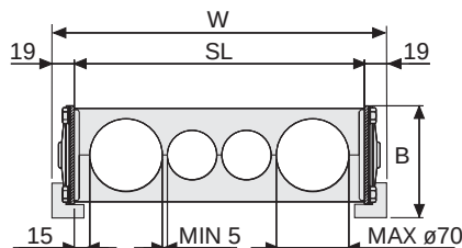
Aluminium Draw Plates with Separators in Nylon
