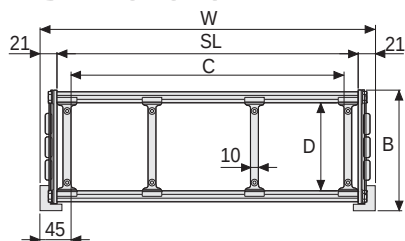
Aluminium Draw Plates with Separators in Nylon
