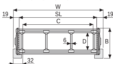
Aluminium Draw Plates with Separators in Nylon
