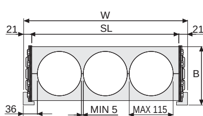
Aluminium Draw Plates with Separators in Nylon
